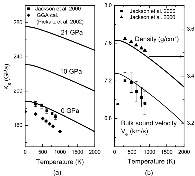
Figure 9. Temperature dependence of (a) adiabatic bulk modulus under various pressure compared with experiments ([Jackson et al. , 2000]) and previous calculation ([Piekarz et al. , 2002]) and (b) bulk sound velocity and density at ambient pressure.
