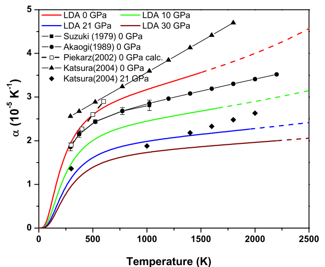
Figure 5. Thermal expansion coefficient along 0, 10, 21, and 30 GPa isobars.
