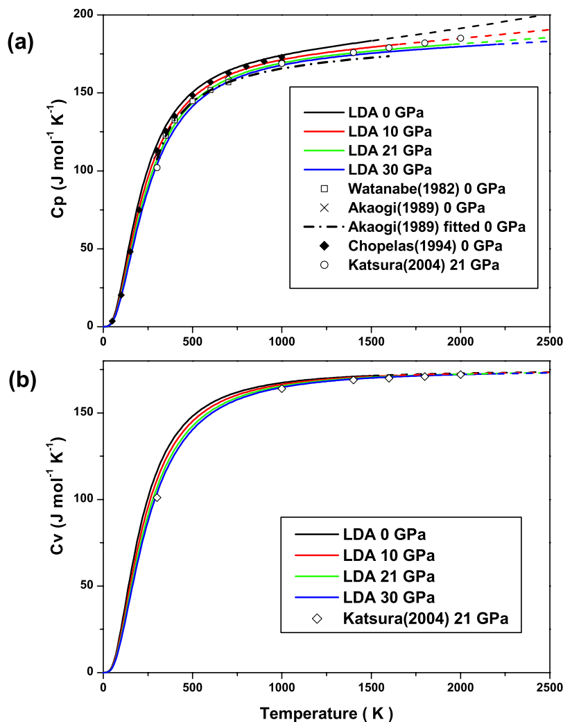
Figure 7. Temperature dependence of specific heat (a) C_p and (b) C_v along the isobars at 0, 10, 21, and 30 GPa. Experimental measurements and fitted results at ambient conditions and high pressures are denoted by symbols and dashed lines [Akaogi et al. , 1984, 1989; Chopelas et al. , 1994; Katsura et al. , 2004].
