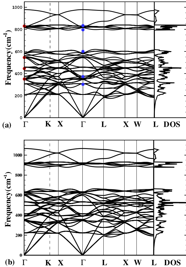
Figure 2. Phonon dispersion and vibrational density of states for \text{Mg}_2\text{SiO}_4 ringwoodite (a) 0 GPa and (b) 20 GPa. Four red dots are from infrared experiments [Chopelas et al. , 1994], and five blue dots represent Raman data [Akaogi et al. , 1984]. These experimental data are also shown in Table 2.
