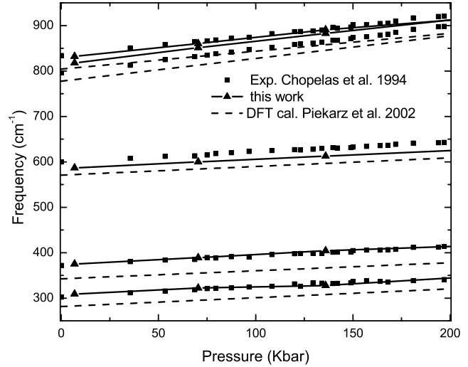
Figure 3. Pressure dependence of the Raman frequencies.
