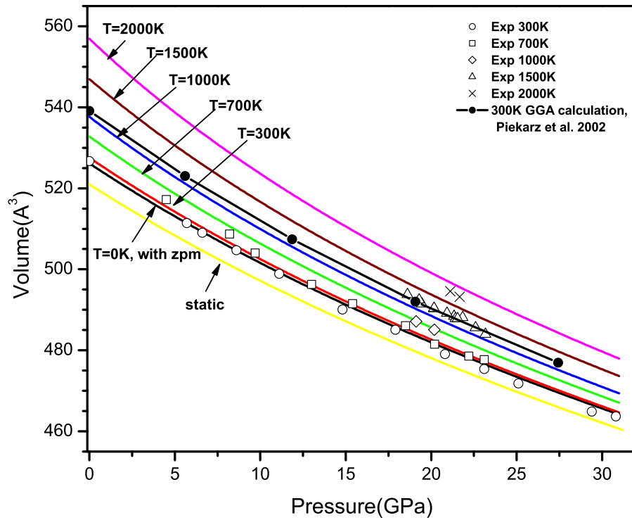
Figure 4. Compression curves for static lattice (without zero point motion) and along 0, 300, 700, 1000, 1500, and 2000 K isotherms. Experimental data at each corresponding temperature are denoted by circles, squares, diamonds, triangles, and crosses, respectively [Katsura et al. , 2004].
