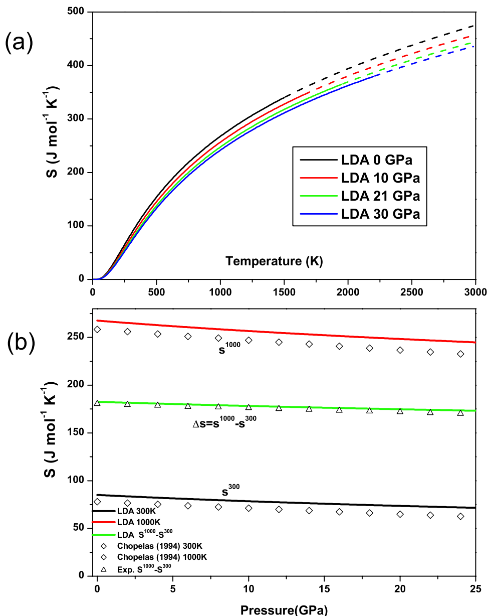
Figure 8. (a) Temperature and (b) pressure dependence of entropy. Symbols represent experimental data [Chopelas et al. , 1994].
