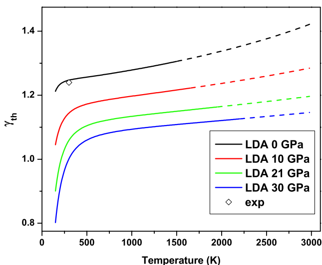
Figure 6. Temperature dependence of the thermal Grüneisen parameter along the isobars at 0, 10, 21, and 30 GPa. Previous result derived from experiment is denoted by diamond [Chopelas et al. , 1994].
