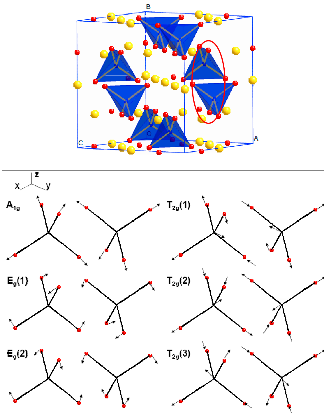
Figure 1. Atomic displacements for the pair of \text{SiO}_4 tetrahedra (in primitive cell) for Raman active modes at 0 GPa in \text{Mg}_2\text{SiO}_4 ringwoodite. Red spheres denote oxygen atoms. At the center of the tetrahedra are Si atoms. The frequency of A_{1g} is 831\text{ cm}^{-1} , E_g(1) and E_g(2) 375\text{ cm}^{-1} , and T_{2g}(1) , T_{2g}(2) , and T_{2g}(3) 817\text{ cm}^{-1} .
